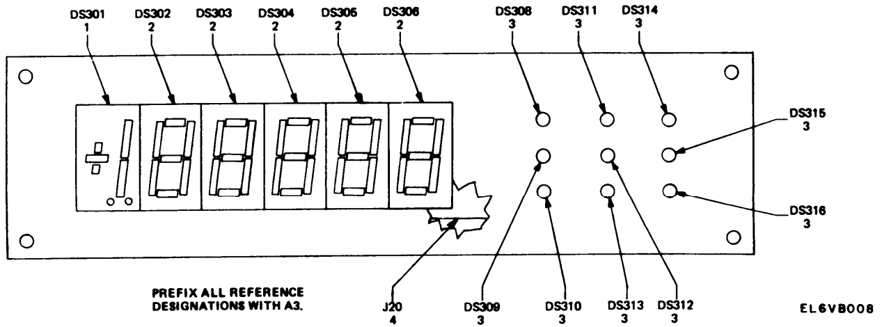
Figure 4. PCB, Display.
