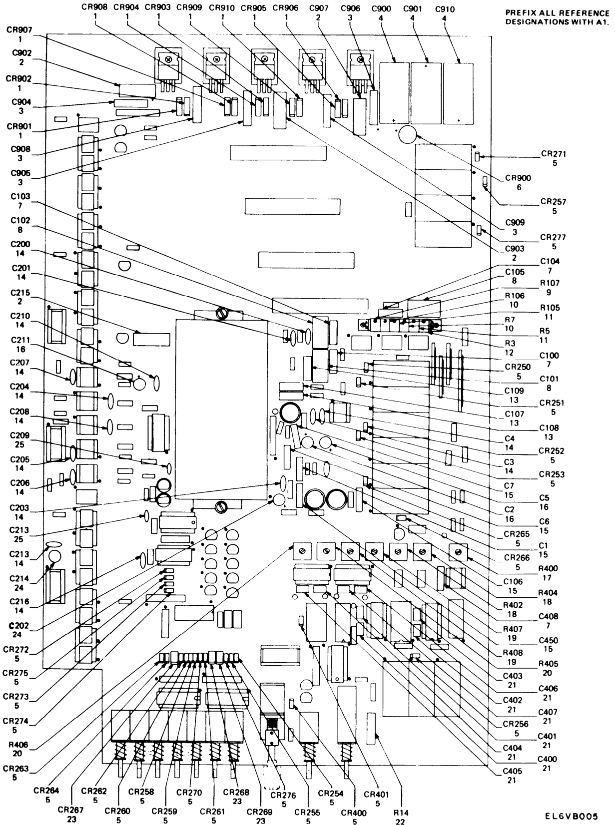
Figure 3. PCB, Analog Motherboard (Sheet 1 of 3).
