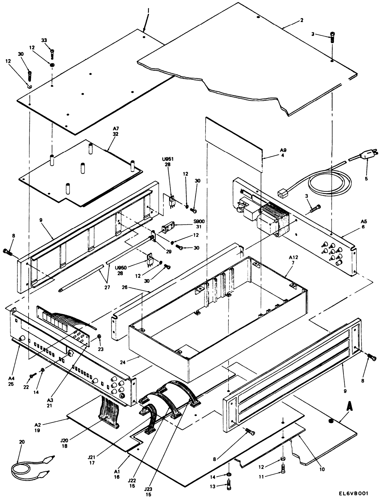
Figure 1. Digital Voltmeter AN/GSM-64C (Sheet 1 of 2).
