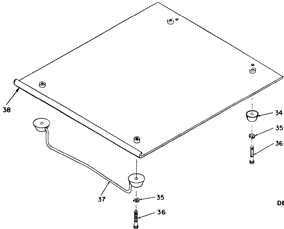
Figure 1. Digital Voltmeter AN/GSM-64C (Sheet 2 of 2).
