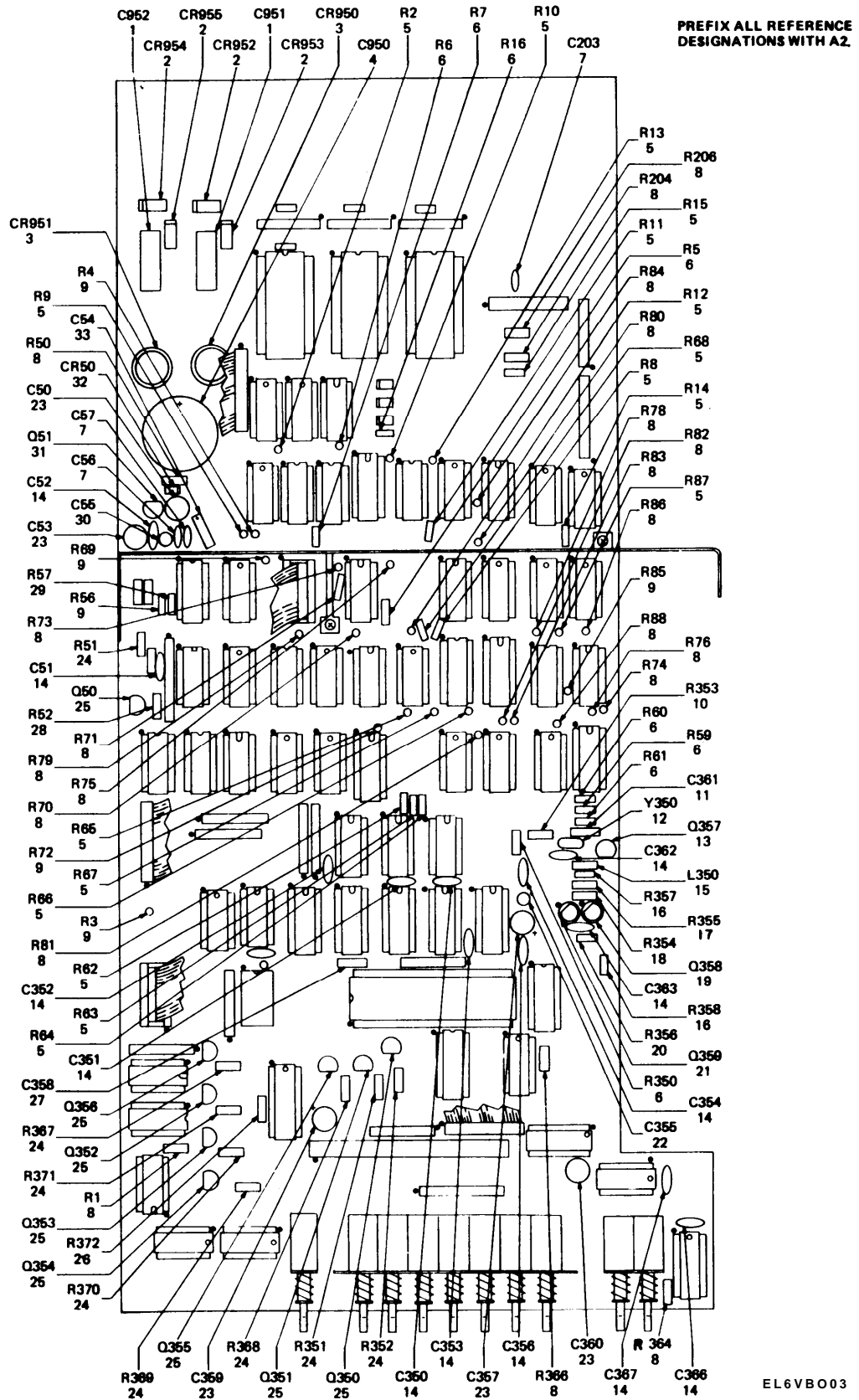
Figure 2. PCB, Digital Motherboard (Sheet 1 of 2).
