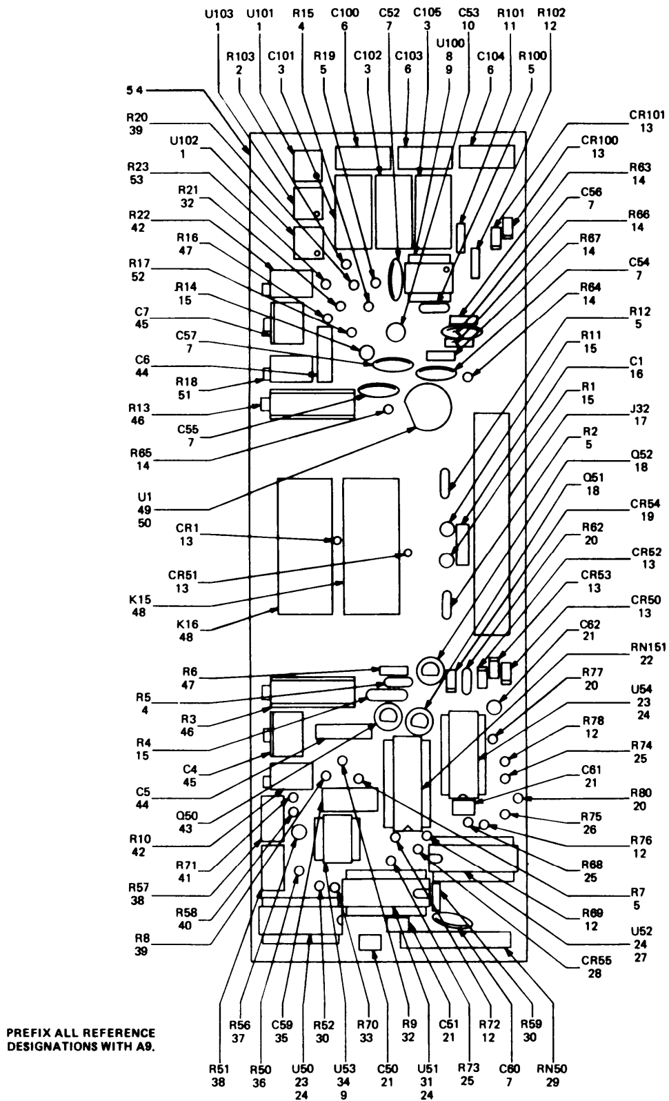
Figure 8. PCB, Dc Ratio.
