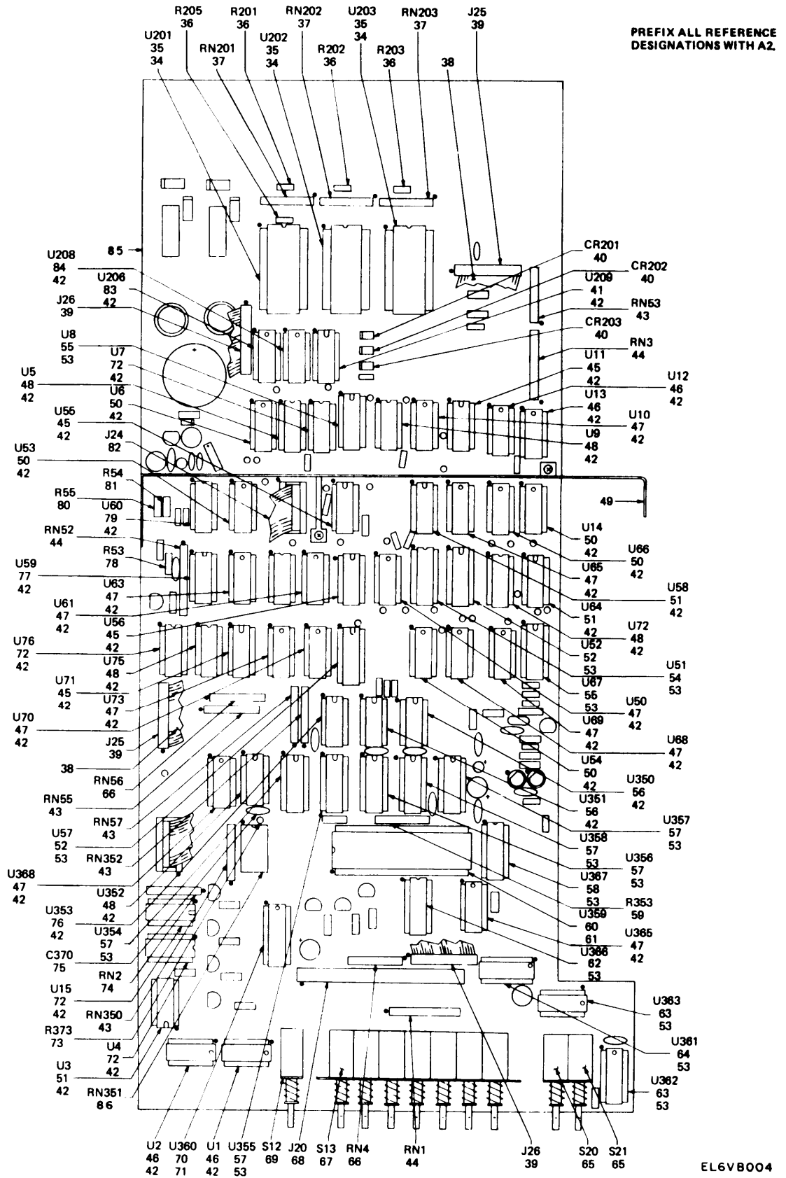
Figure 2. PCB, Digital Motherboard (Sheet 2 of 2).
