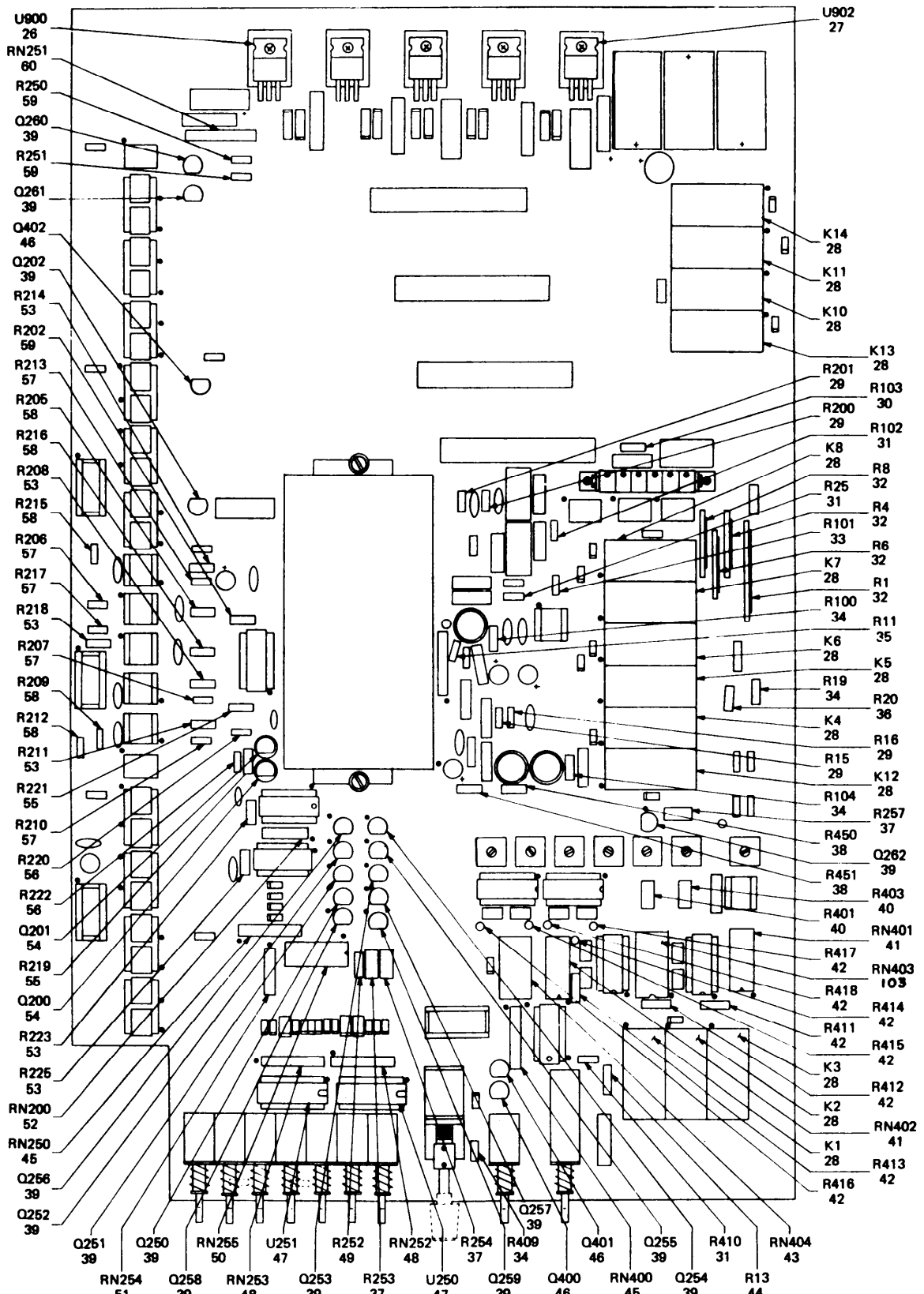
PCB, Analog Motherboard (Sheet 2 of 3).
