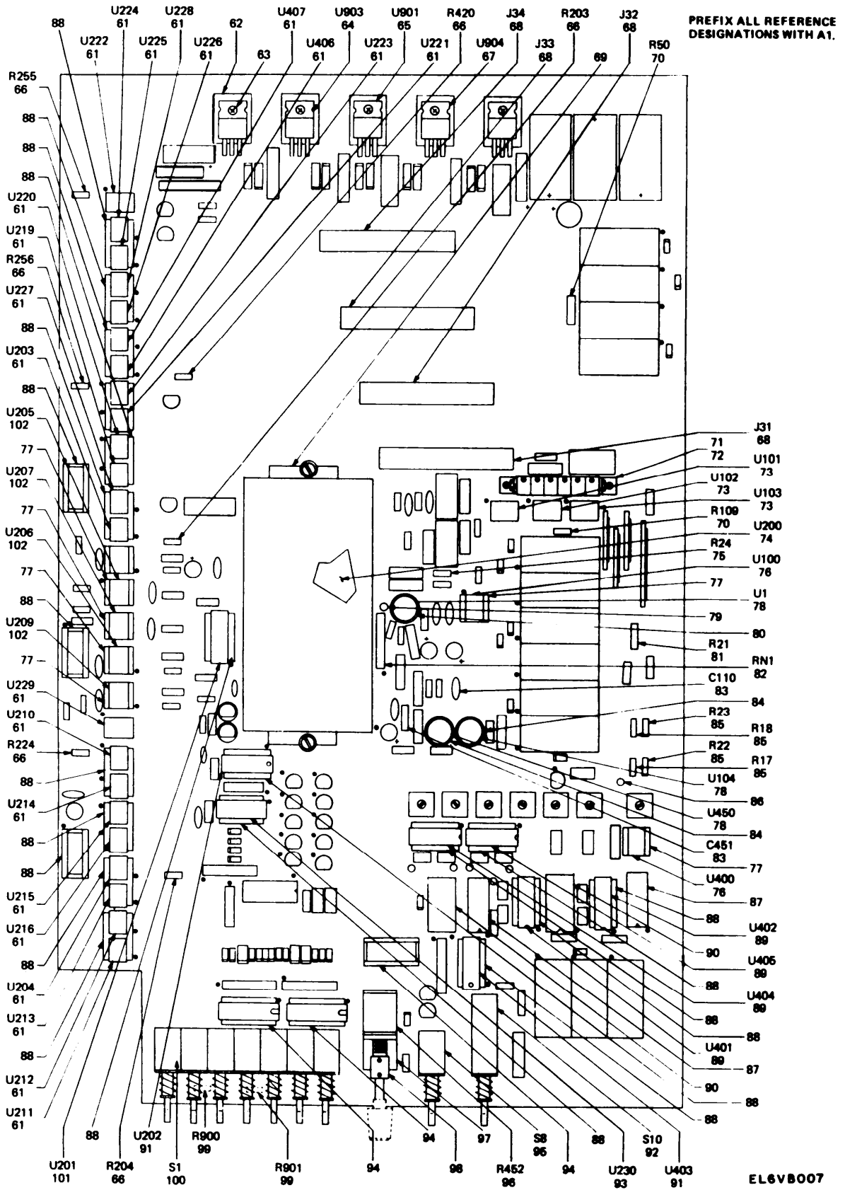
Figure 3. PCB, Analog Motherboard (Sheet 3 of 3)
